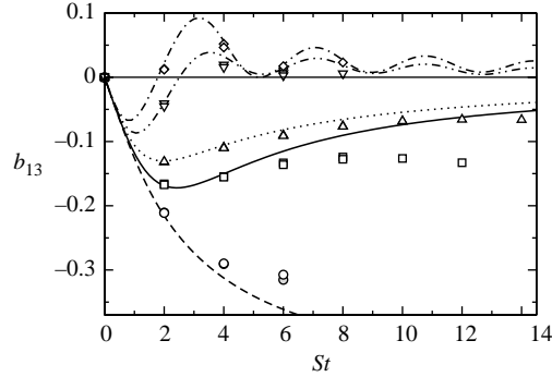
FIGURE 5. Time development of the Reynolds stress anisotropy component b_{13} . Symbols and lines as in figure 3.
