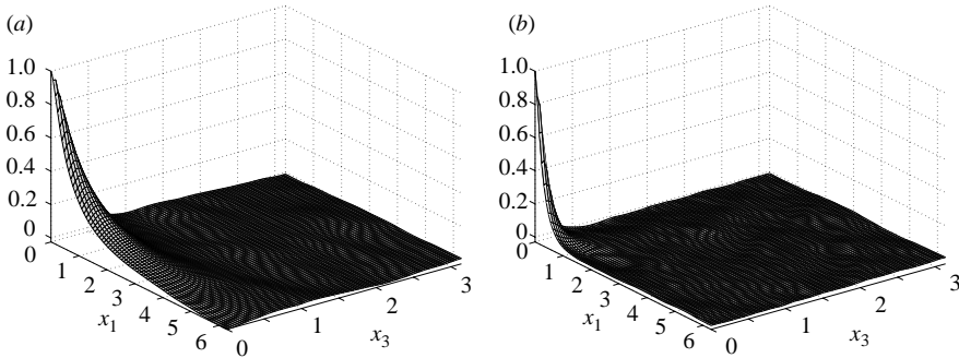
FIGURE 17. The two-point correlations (a) \rho[u_3](\mathbf{r}) and (b) \rho[u_1](\mathbf{r}) at R=-1 and St=14 , series B, for separation vectors in the (x_1, x_3) -plane. Here, u_3 is almost parallel to the principal axis of the Reynolds stress tensor and u_1 is perpendicular.
