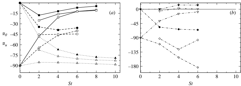
FIGURE 30. Time development of \alpha_u (open symbols) and \alpha_\theta for \theta_1 (filled symbols) and \theta_3 (grey symbols), extracted from the DNS. (a) shows the results of the cases ( \square — \square ), R=0 ; ( \circ — \circ ), R=-1/2 ; ( \triangle ··· \triangle ), R=-1 ; and (b) shows the results of the cases ( \nabla — \nabla ), R=1/2 ; ( \diamond — \diamond ), R=-3/2 .
