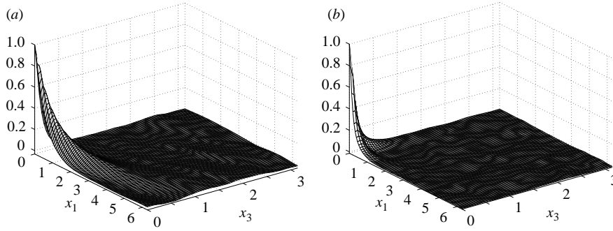
FIGURE 15. The two-point correlations (a) \rho[u_1](\mathbf{r}) and (b) \rho[u_3](\mathbf{r}) at R=0 and St=12 , series B , for separation vectors in the (x_1, x_3) -plane. Here, u_1 is almost parallel to the principal axis of the Reynolds stress tensor and u_3 perpendicular.
