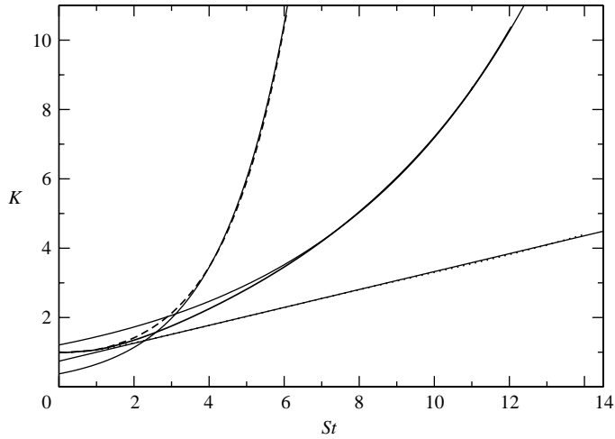
FIGURE 4. Time development of the turbulent kinetic energy K according to DNS, series B . -\text{---} , (thick line) R=0 ; -\text{---} , R=-1/2 ; \cdots , R=-1 . The thin solid lines are fitted exponential functions at R=0 ( \exp(0.178St) ) and R=-1/2 ( \exp(0.56St) ) and a linear fit at R=-1 .
