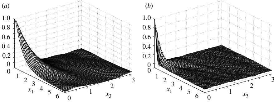
FIGURE 16. The two-point correlations (a) \rho[u](\mathbf{r}) and (b) \rho[w](\mathbf{r}) at R=-1/2 and St=6 , series A, for separation vectors in the (x_1, x_3) -plane. Here, u = u_1 \cos \alpha_u + u_3 \sin \alpha_u , w = -u_1 \sin \alpha_u + u_3 \cos \alpha_u and \alpha_u = -45^\circ . Thus, u is the strongest fluctuating velocity component and is parallel to the principal axis of the Reynolds stress tensor and w perpendicular.
