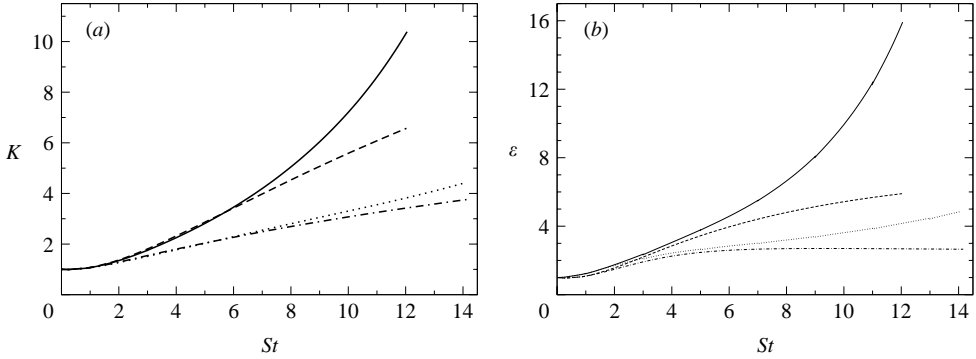
FIGURE 13. Time development of (a) K and (b) \varepsilon at R=0 series B (—) and R=-1 series B ( \cdots ) and the corresponding simulations without the nonlinear terms at R=0 (---) and at R=-1 (-·-·).
